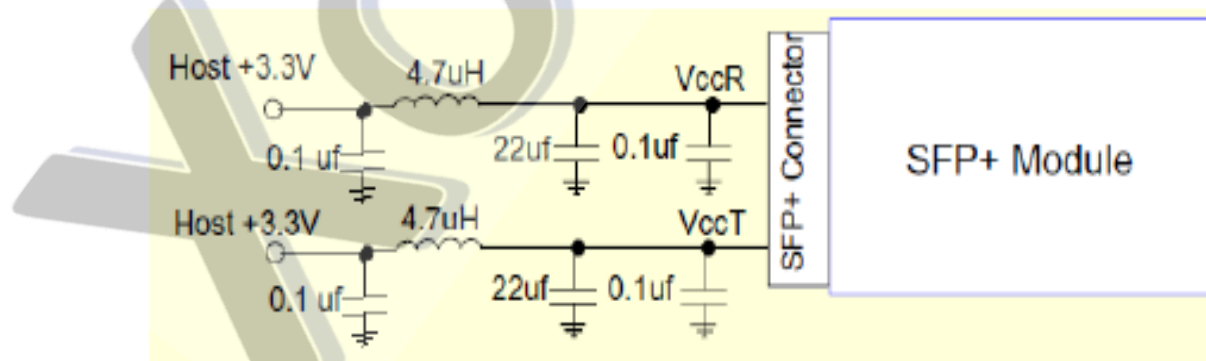
Recommended Host Board Power Supply Circuit
